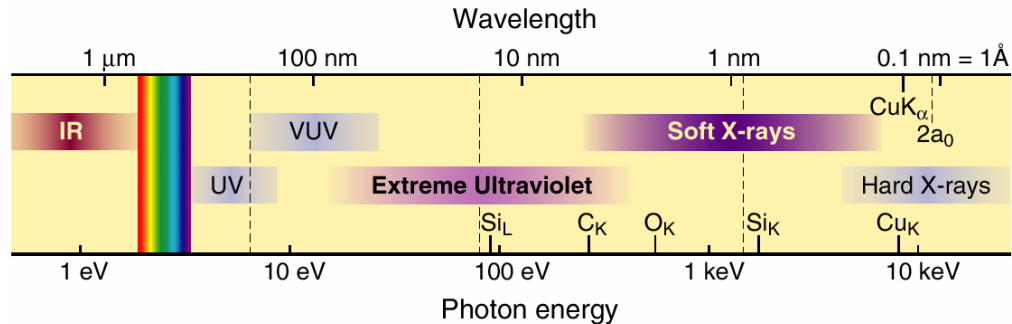
Figure 1.5.1. The short wavelength region of the electromagnetic spectrum, taken from ref. 74. Here, one can see that O K edge ( \sim 540 eV) and Cu L 2,3 edges ( \sim 932 eV and 952 eV) are lying in the soft X-ray range.
