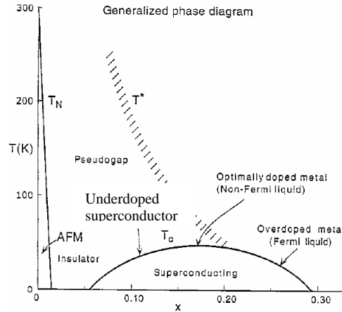
Figure 1.2.2 Generic phase diagram of doped hole cuprates superconductors [35].
