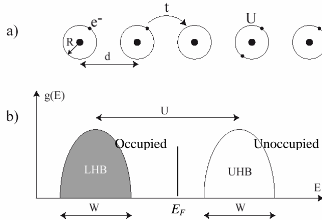
Figure 1.1.1 (a) one dimensional hydrogen chain. R denotes the radius of a 1s Bohr orbit, d is the interatomic spacing (b) Density of state for half filled one band Hubbard model for U > W . In one dimension W = 4t and in two-dimensional W = 8t for a square lattice.
