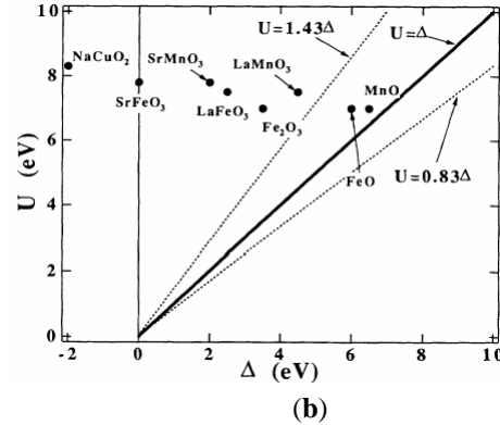
Figure 1.1.3 Zaanen-Sawatzky Allen \Delta - U diagram for (a) divalent and (b) higher valent transition metal compounds study by ref. [26]. The regime above the line U=\Delta is the charge transfer regime while the regime below this line is the Mott-Hubbard regime.
