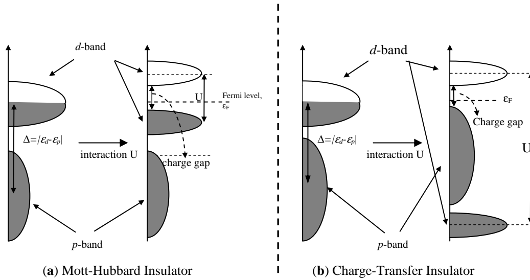
Figure 1.1.2 (a) Schematic band structure of a Mott Hubbard insulator. The p -band lies before the d -band, and the low energy charge excitations occur between the lower and upper Hubbard band. (b) Schematic band structure of a Charge-Transfer insulator. The p -band lies between the lower and upper Hubbard band. The lower energy charge excitation involves the d and p -bands.
