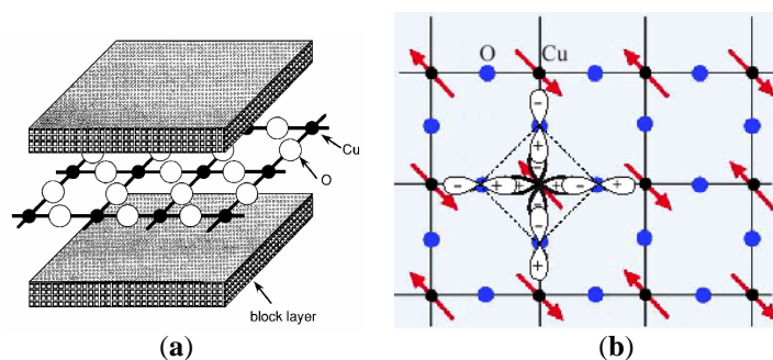
Figure 1.2.1 (a) Conceptual illustration of staking of CuO 2 layers sandwiched by block layers. (b) Schematic of CuO 2 plane.
